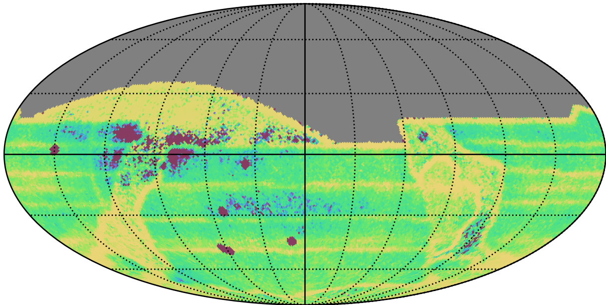
early_u_fpextra3.0_v3.4_10yrs All sky: Median Intra-Night Gap
