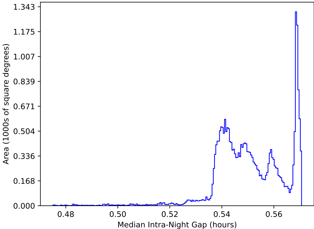
early_u_fpextra3.0_v3.4_10yrs All sky: Median Intra-Night Gap
