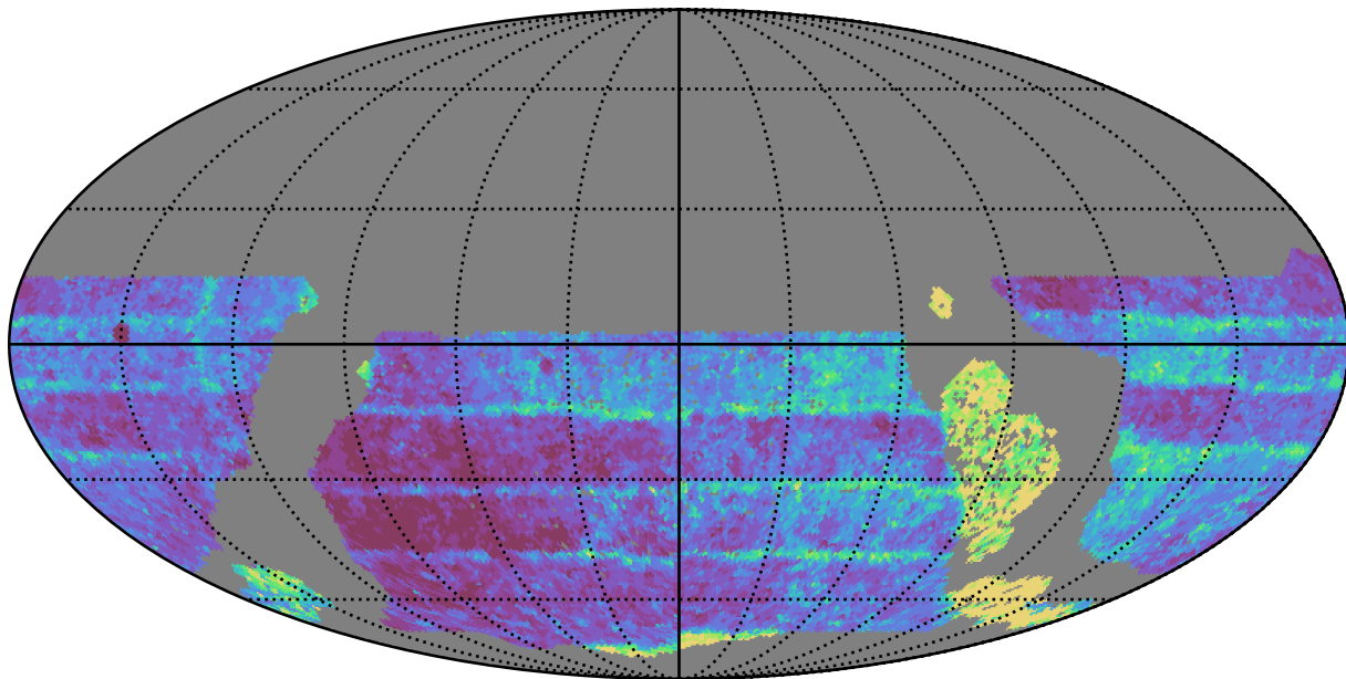
early_u_fpextra3.0_v3.4_10yrs WFD z band: Median Inter-Night Gap
