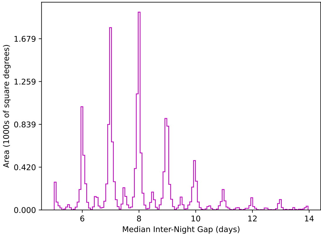
early_u_fpextra3.0_v3.4_10yrs WFD z band: Median Inter-Night Gap
