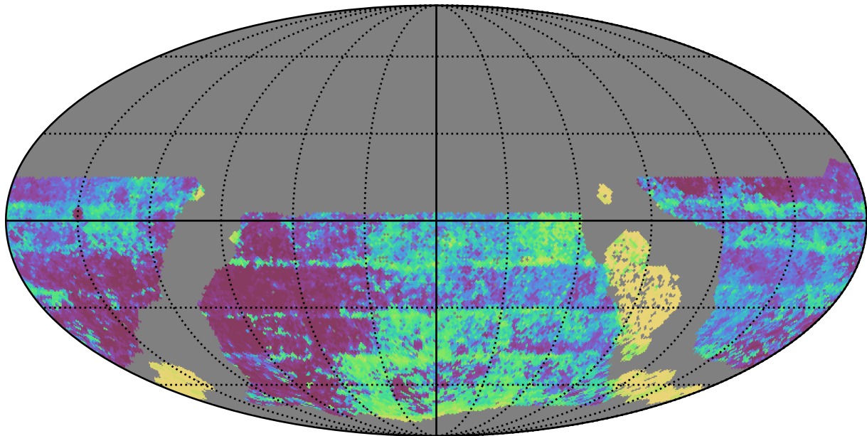
early_u_fpextra3.0_v3.4_10yrs WFD y band: Median Inter-Night Gap
