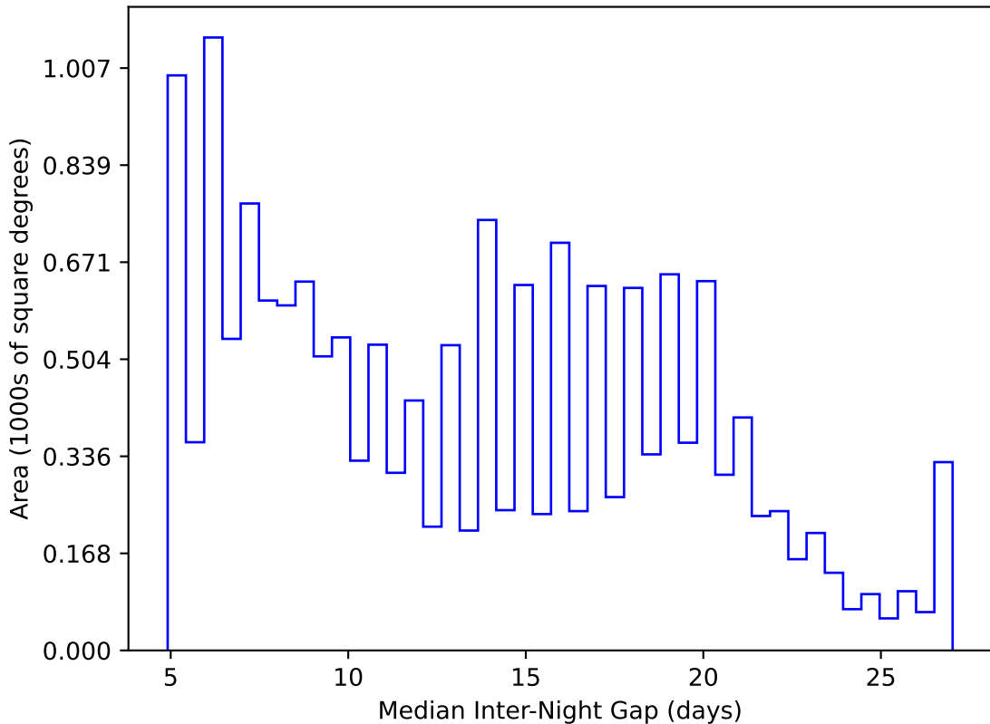
early_u_fpextra3.0_v3.4_10yrs WFD y band: Median Inter-Night Gap
