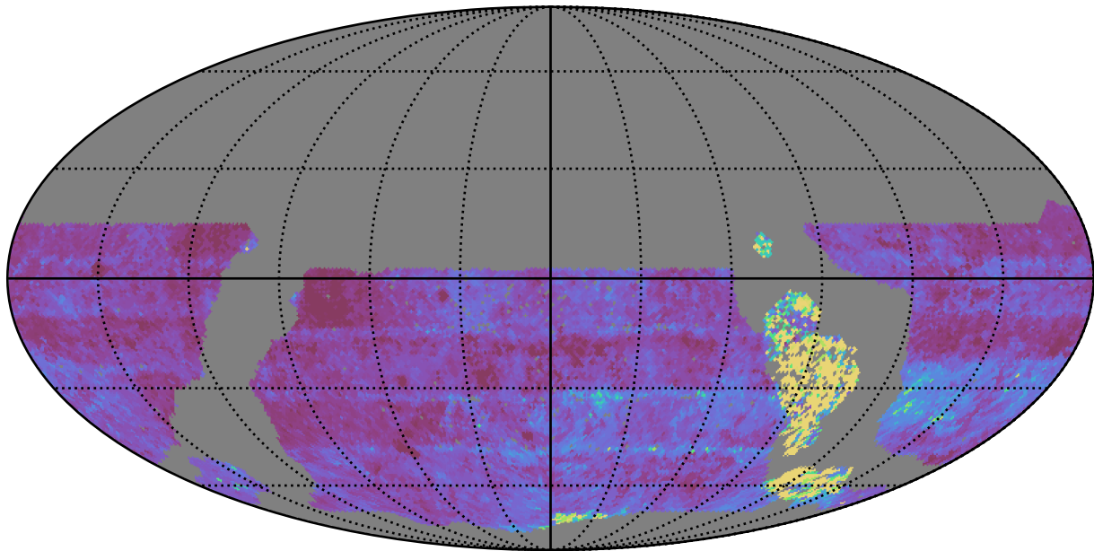
early_u_fpextra3.0_v3.4_10yrs WFD u band: Median Inter-Night Gap
