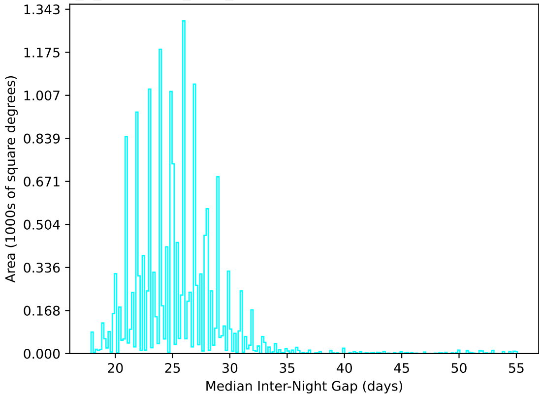
early_u_fpextra3.0_v3.4_10yrs WFD u band: Median Inter-Night Gap
