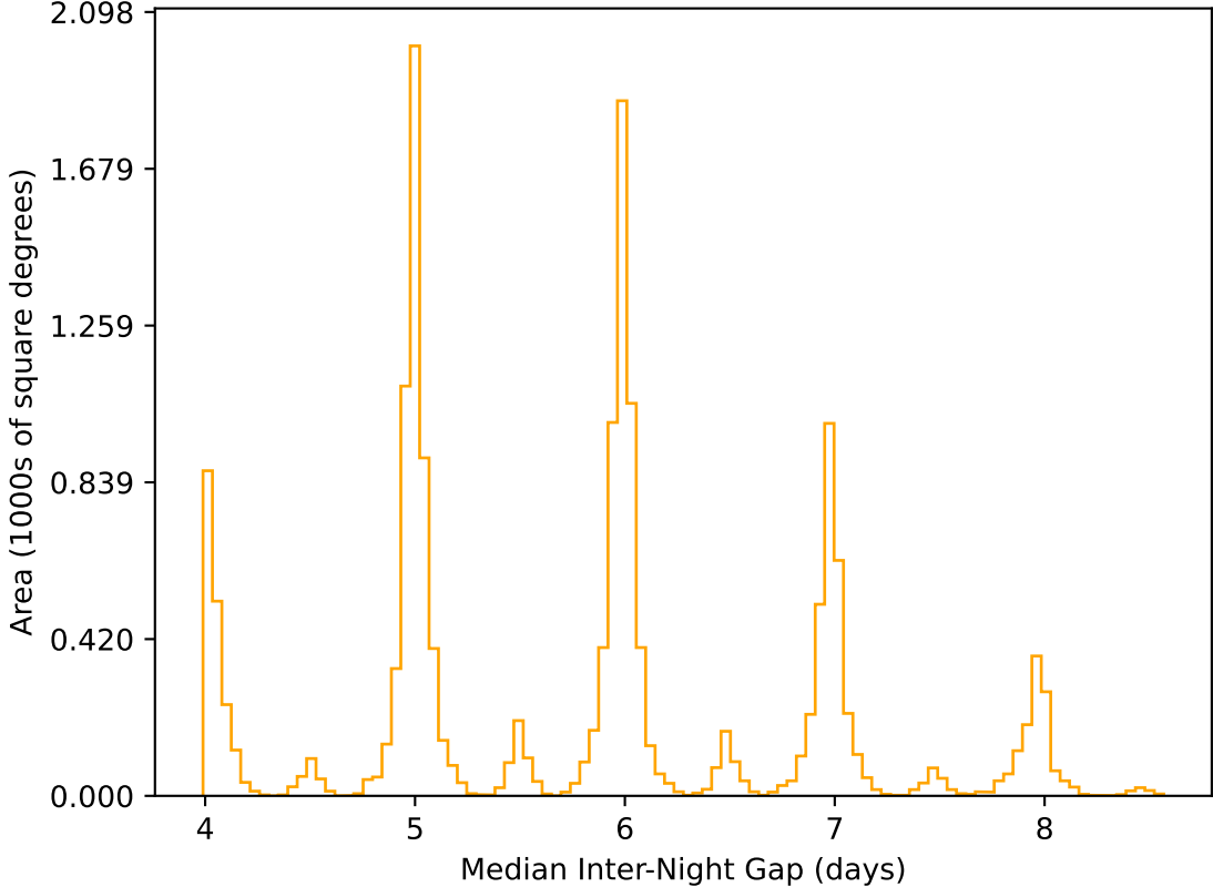
early_u_fpextra3.0_v3.4_10yrs WFD r band: Median Inter-Night Gap
