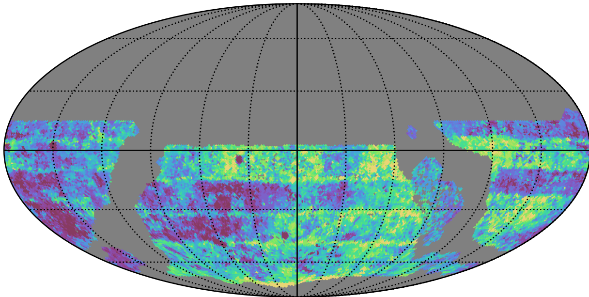
early_u_fpextra3.0_v3.4_10yrs WFD g band: Median Inter-Night Gap
