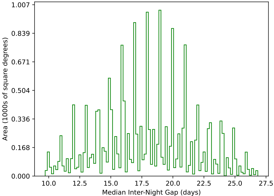
early_u_fpextra3.0_v3.4_10yrs WFD g band: Median Inter-Night Gap
