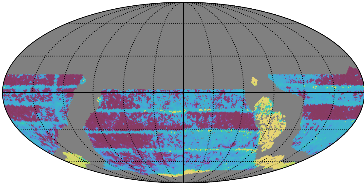
early_u_fpextra3.0_v3.4_10yrs WFD all bands: Median Inter-Night Gap
