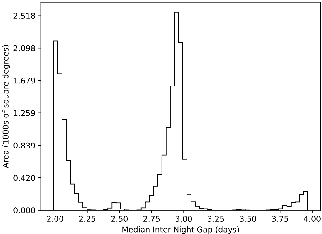
early_u_fpextra3.0_v3.4_10yrs WFD all bands: Median Inter-Night Gap
