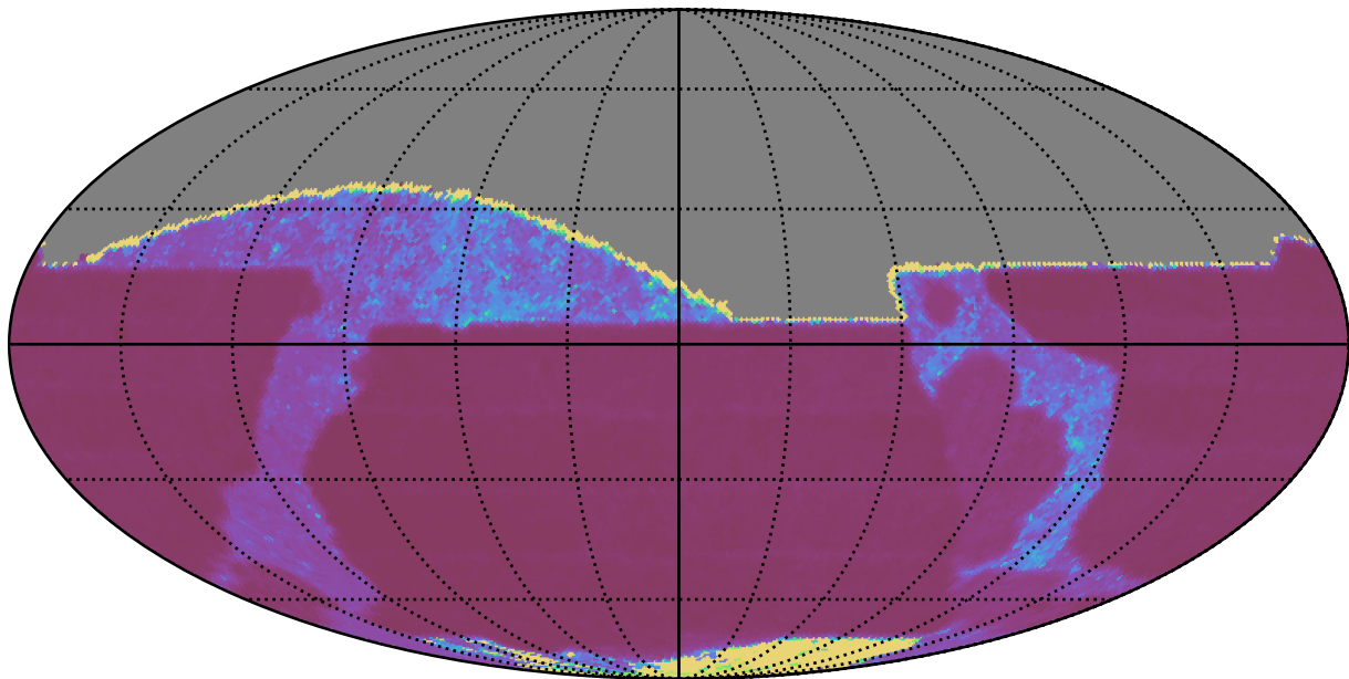
early_u_fpextra3.0_v3.4_10yrs All sky z band: Median Inter-Night Gap
