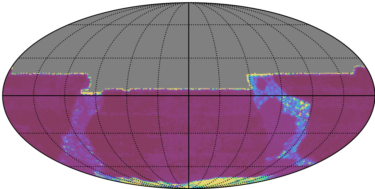
early_u_fpextra3.0_v3.4_10yrs All sky y band: Median Inter-Night Gap
