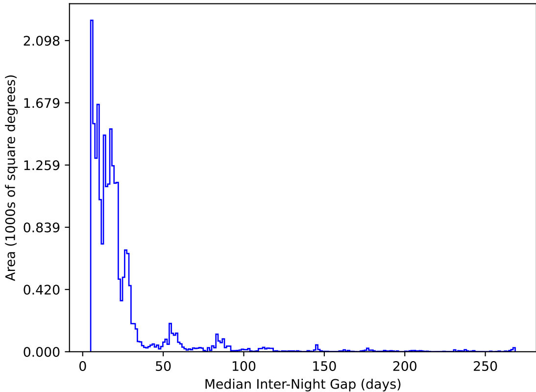
early_u_fpextra3.0_v3.4_10yrs All sky y band: Median Inter-Night Gap
