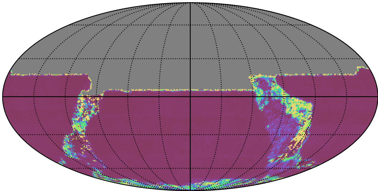
early_u_fpextra3.0_v3.4_10yrs All sky u band: Median Inter-Night Gap
