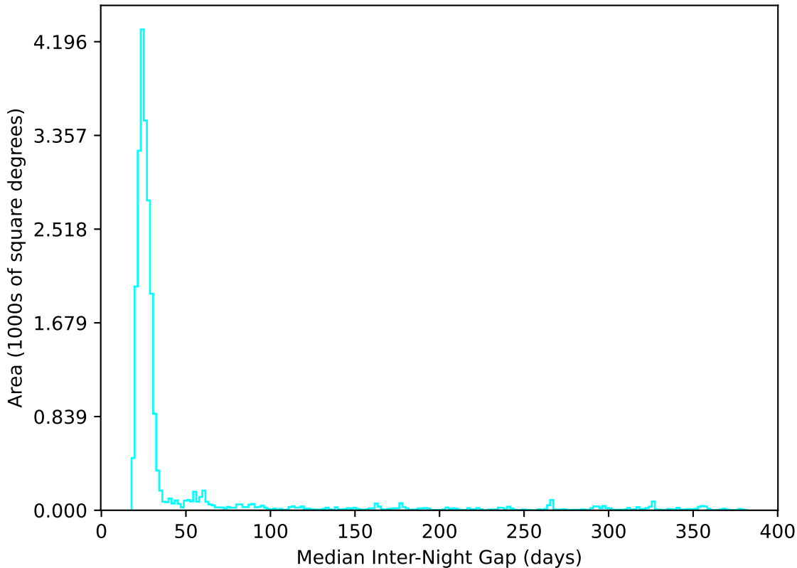
early_u_fpextra3.0_v3.4_10yrs All sky u band: Median Inter-Night Gap
