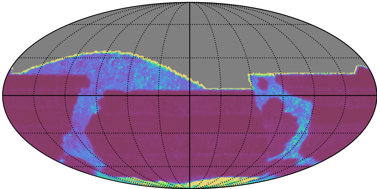
early_u_fpextra3.0_v3.4_10yrs All sky r band: Median Inter-Night Gap
