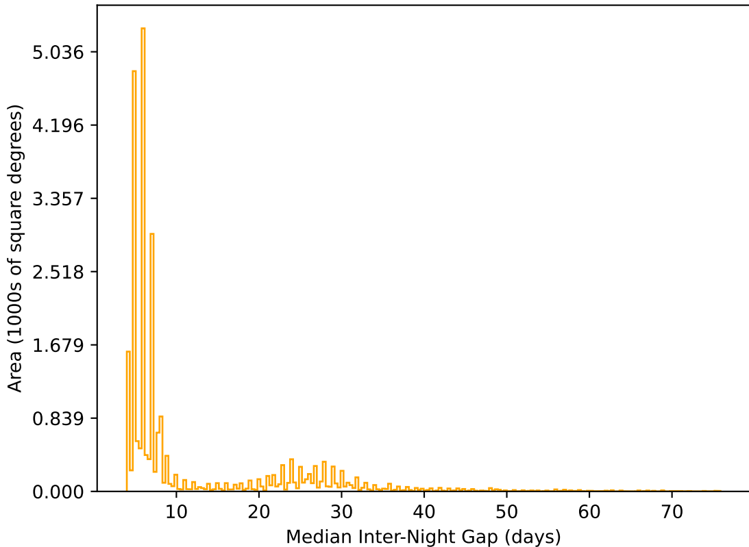
early_u_fpextra3.0_v3.4_10yrs All sky r band: Median Inter-Night Gap
