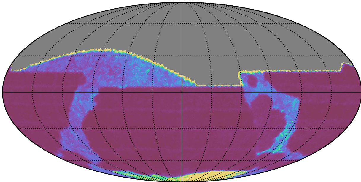
early_u_fpextra3.0_v3.4_10yrs All sky i band: Median Inter-Night Gap
