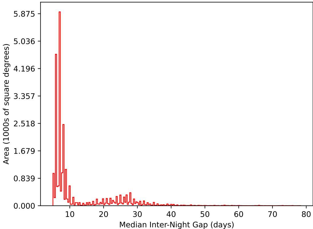
early_u_fpextra3.0_v3.4_10yrs All sky i band: Median Inter-Night Gap
