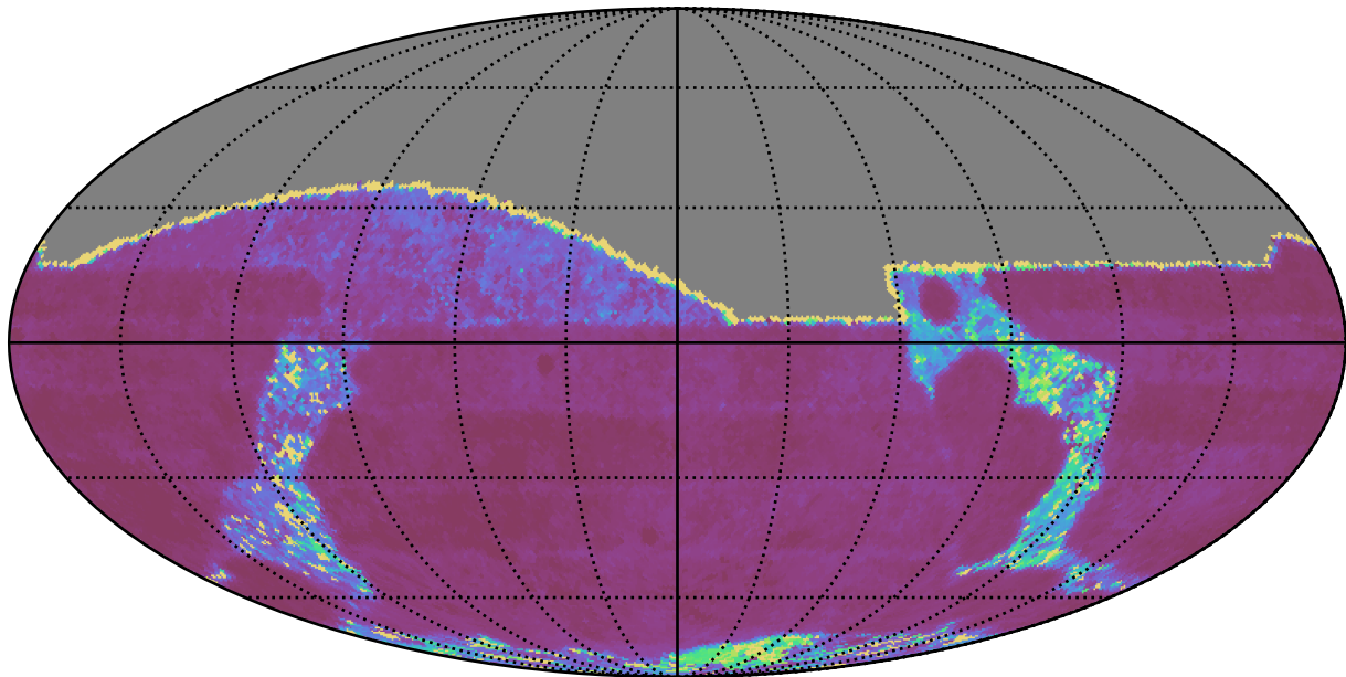
early_u_fpextra3.0_v3.4_10yrs All sky g band: Median Inter-Night Gap
