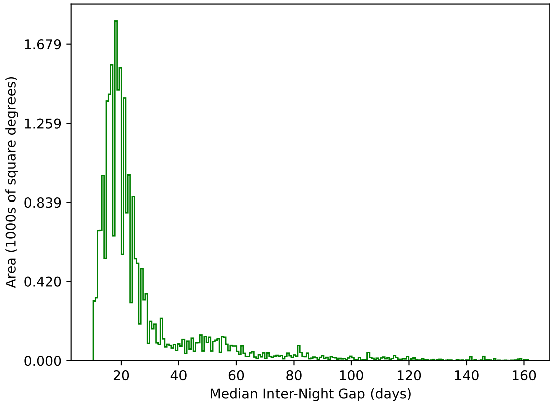
early_u_fpextra3.0_v3.4_10yrs All sky g band: Median Inter-Night Gap
