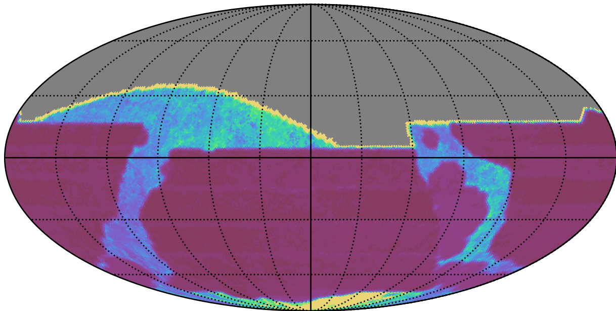
early_u_fpextra3.0_v3.4_10yrs All sky all bands: Median Inter-Night Gap
