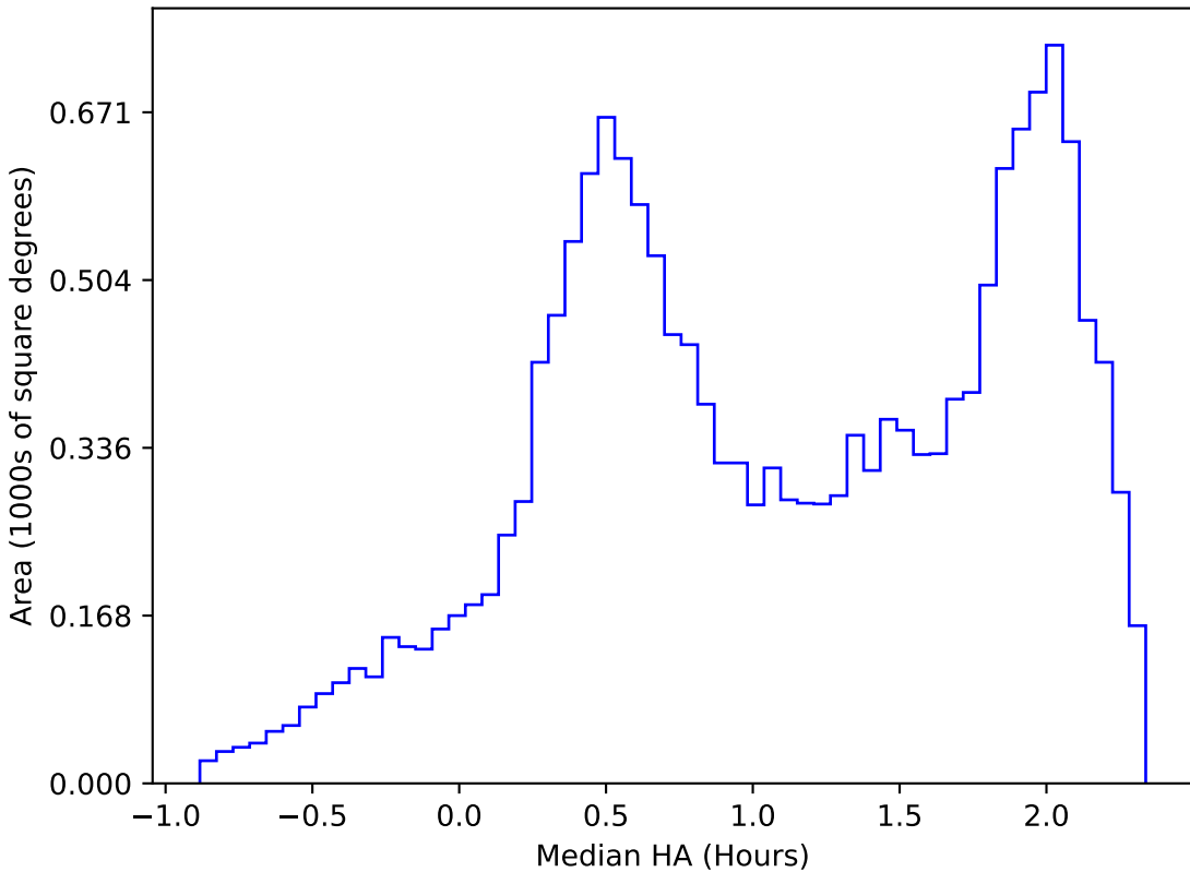
early_u_fpextra3.0_v3.4_10yrs WFD z band: Median HA
