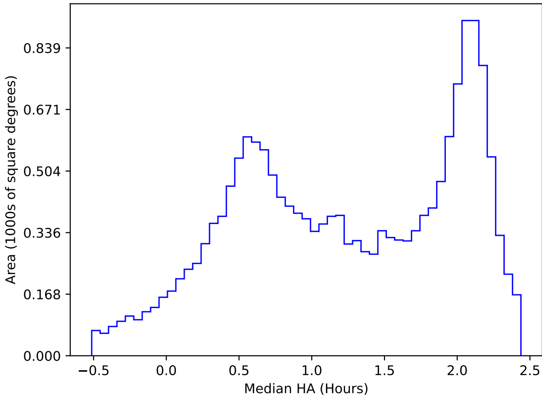
early_u_fpextra3.0_v3.4_10yrs WFD y band: Median HA
