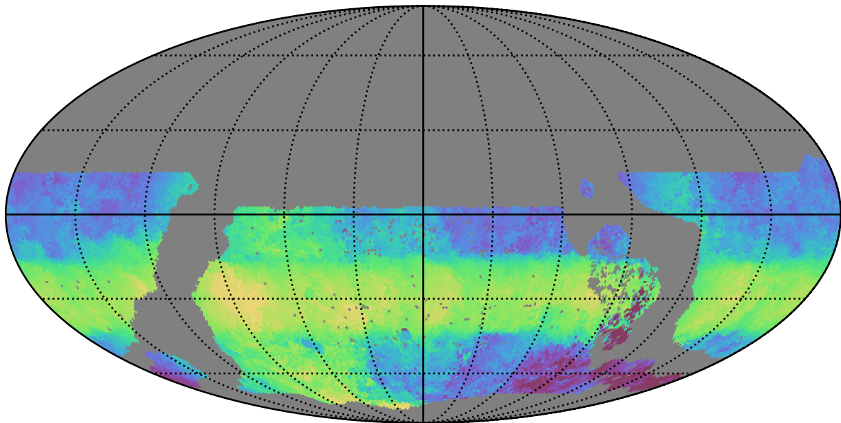
early_u_fpextra3.0_v3.4_10yrs WFD u band: Median HA
