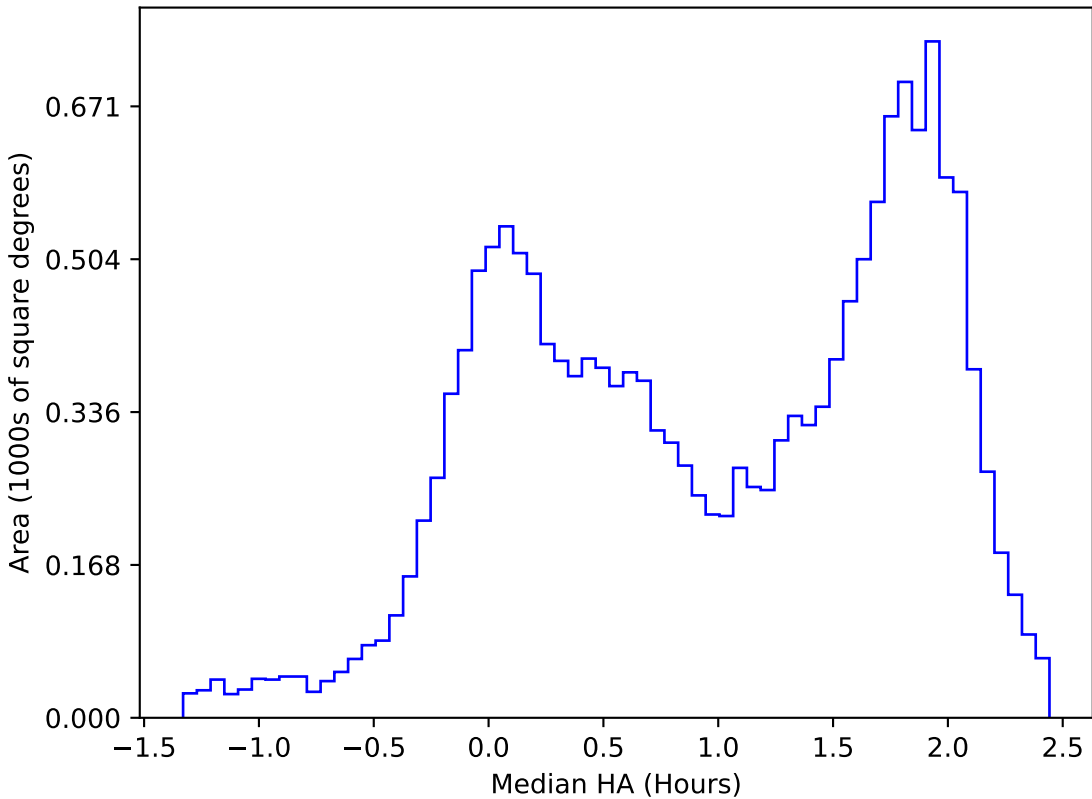
early_u_fpextra3.0_v3.4_10yrs WFD u band: Median HA
