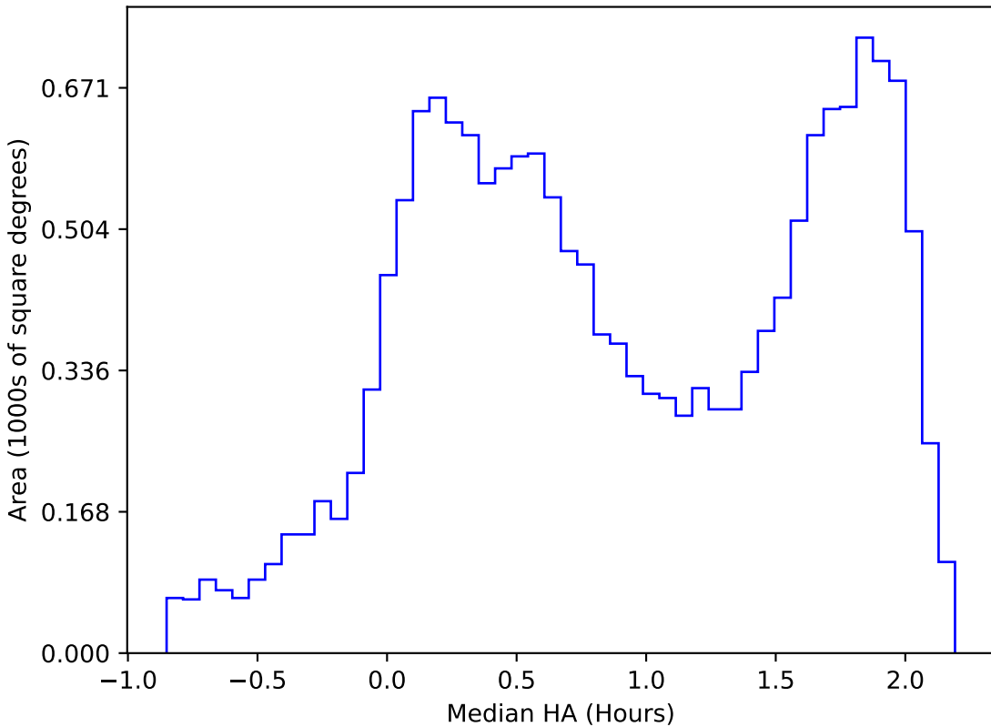
early_u_fpextra3.0_v3.4_10yrs WFD r band: Median HA
