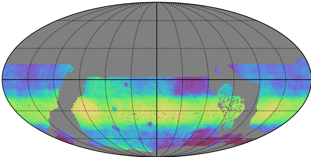
early_u_fpextra3.0_v3.4_10yrs WFD i band: Median HA
