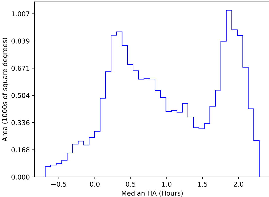
early_u_fpextra3.0_v3.4_10yrs WFD i band: Median HA
