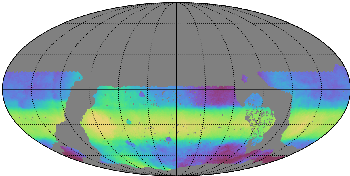
early_u_fpextra3.0_v3.4_10yrs WFD all bands: Median HA
