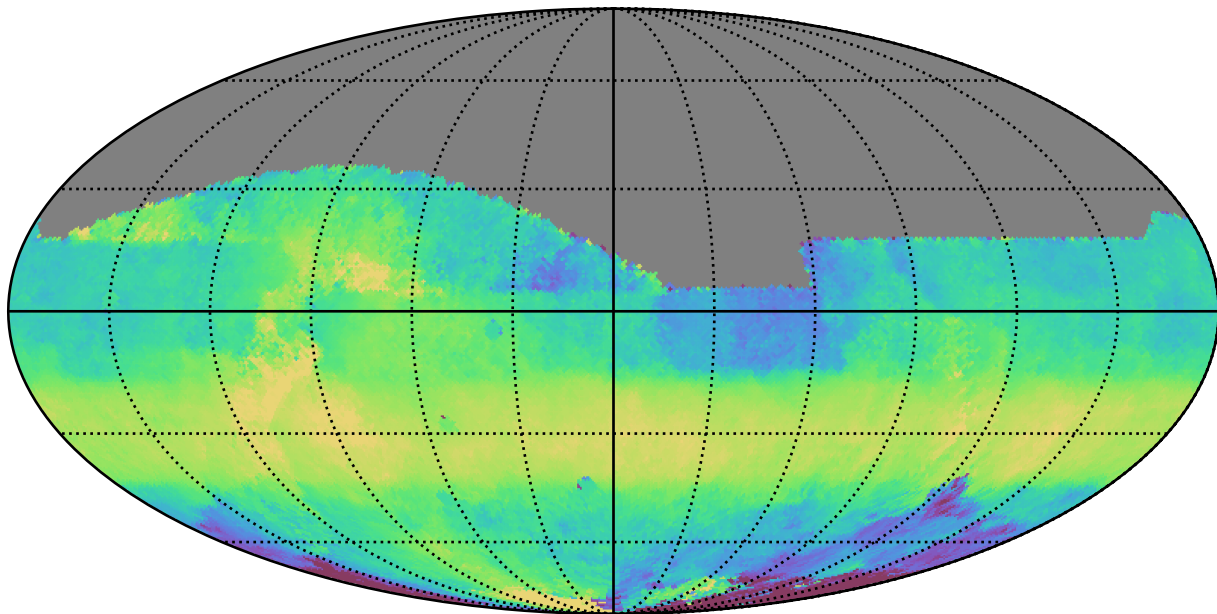
early_u_fpextra3.0_v3.4_10yrs All sky z band: Median HA
