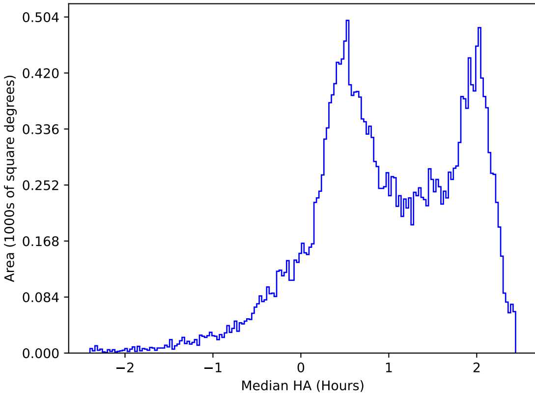
early_u_fpextra3.0_v3.4_10yrs All sky z band: Median HA
