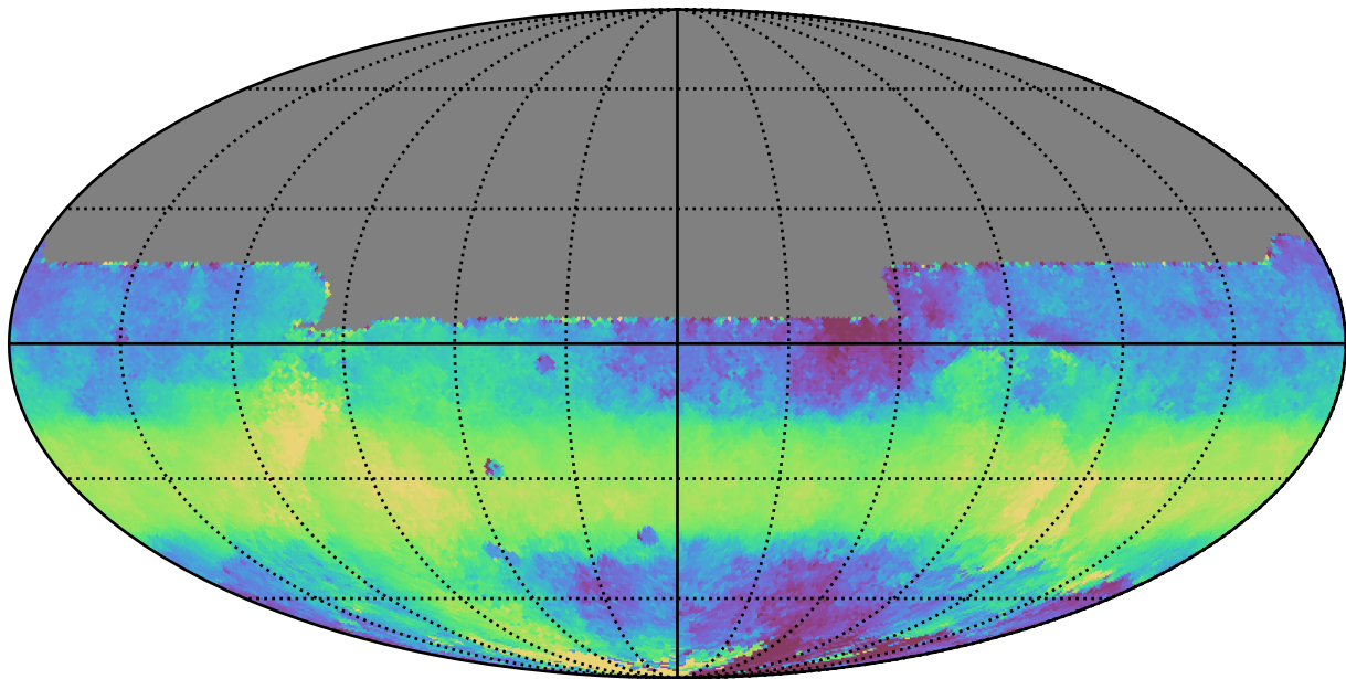
early_u_fpextra3.0_v3.4_10yrs All sky y band: Median HA
