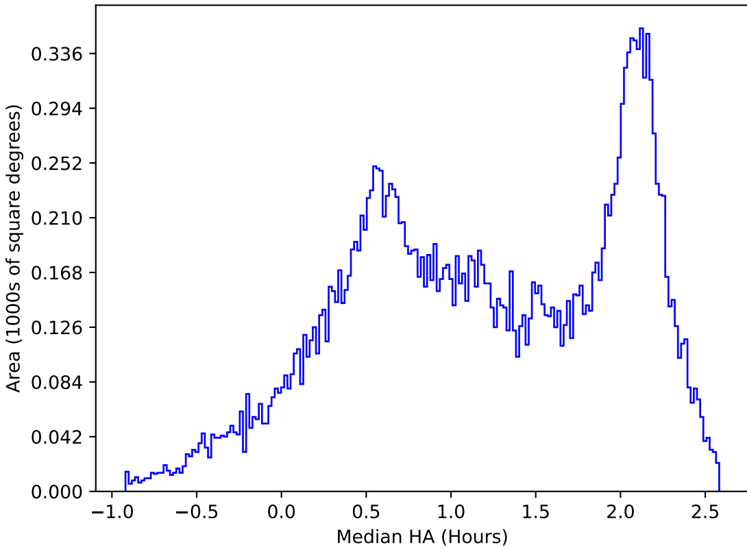
early_u_fpextra3.0_v3.4_10yrs All sky y band: Median HA
