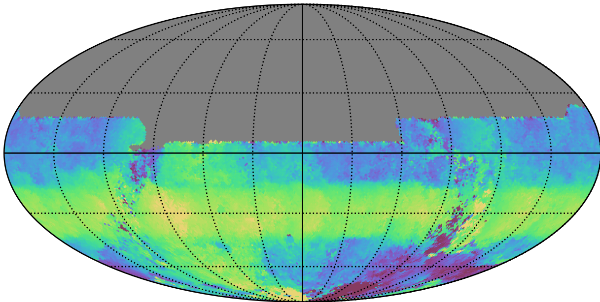
early_u_fpextra3.0_v3.4_10yrs All sky u band: Median HA
