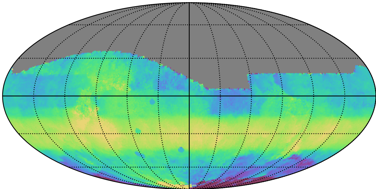
early_u_fpextra3.0_v3.4_10yrs All sky i band: Median HA
