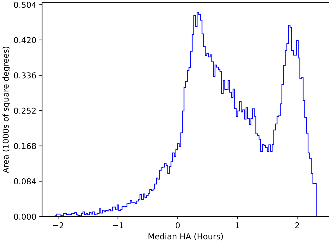
early_u_fpextra3.0_v3.4_10yrs All sky i band: Median HA
