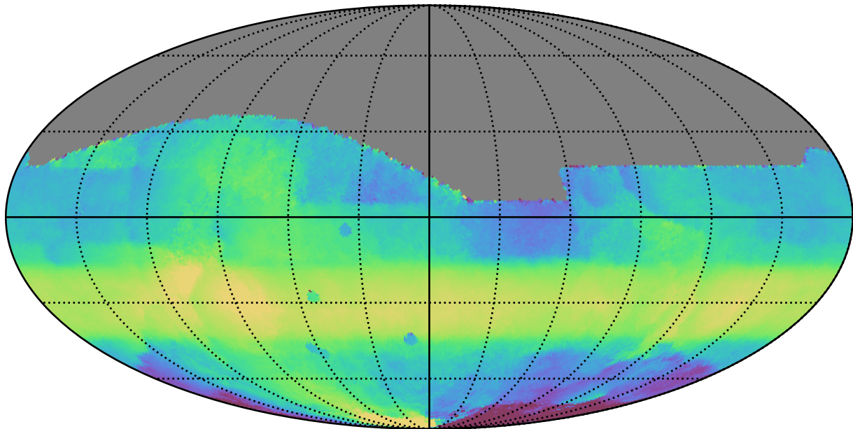
early_u_fpextra3.0_v3.4_10yrs All sky all bands: Median HA
