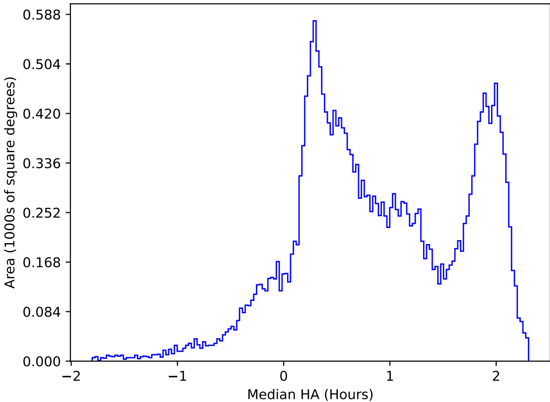
early_u_fpextra3.0_v3.4_10yrs All sky all bands: Median HA
