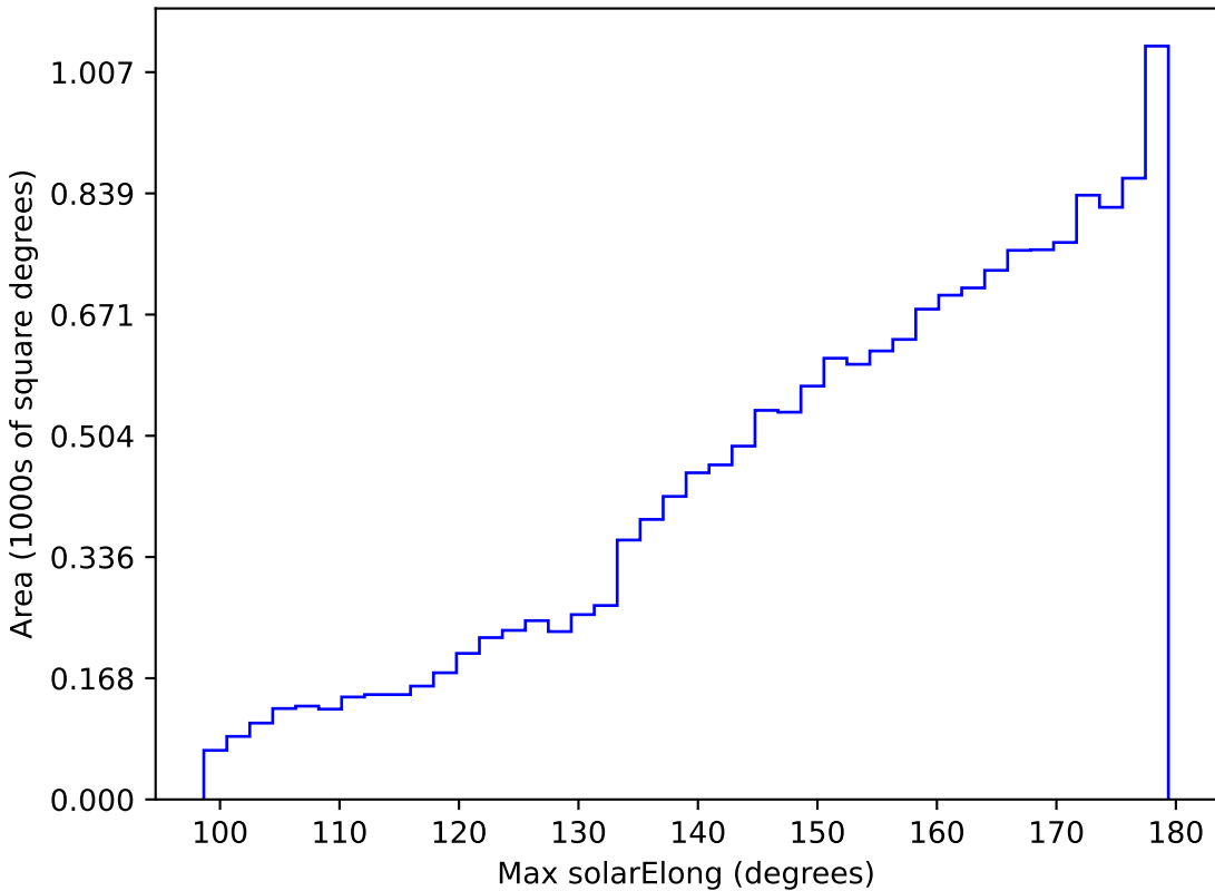
early_u_fpextra3.0_v3.4_10yrs WFD z band: Max solarElong
