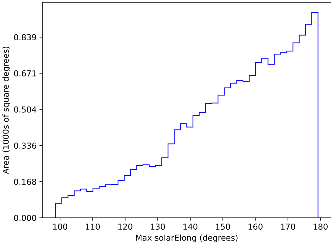
early_u_fpextra3.0_v3.4_10yrs WFD y band: Max solarElong
