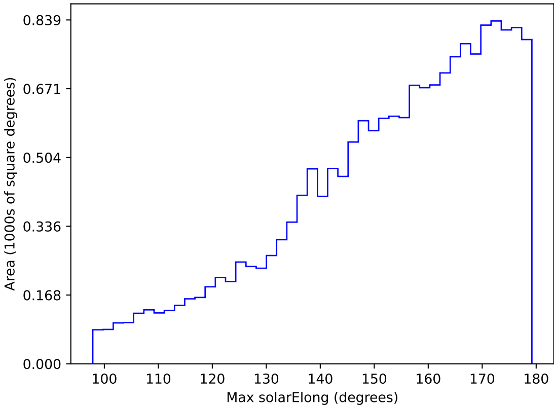
early_u_fpextra3.0_v3.4_10yrs WFD u band: Max solarElong
