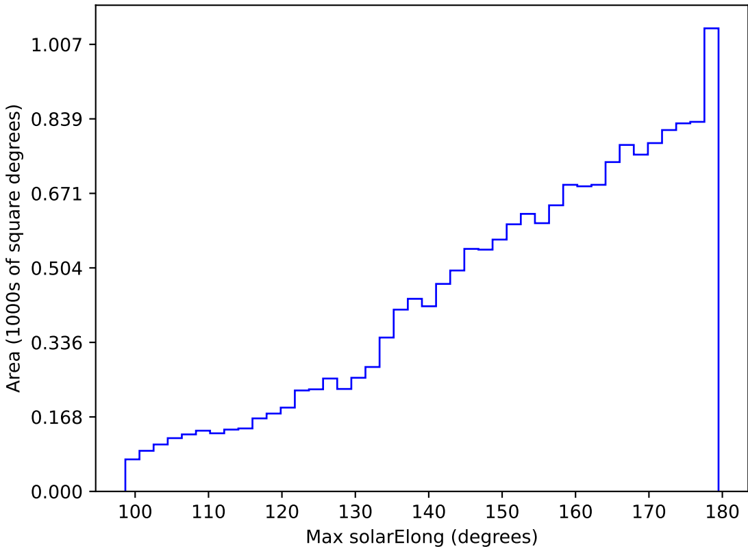
early_u_fpextra3.0_v3.4_10yrs WFD r band: Max solarElong
