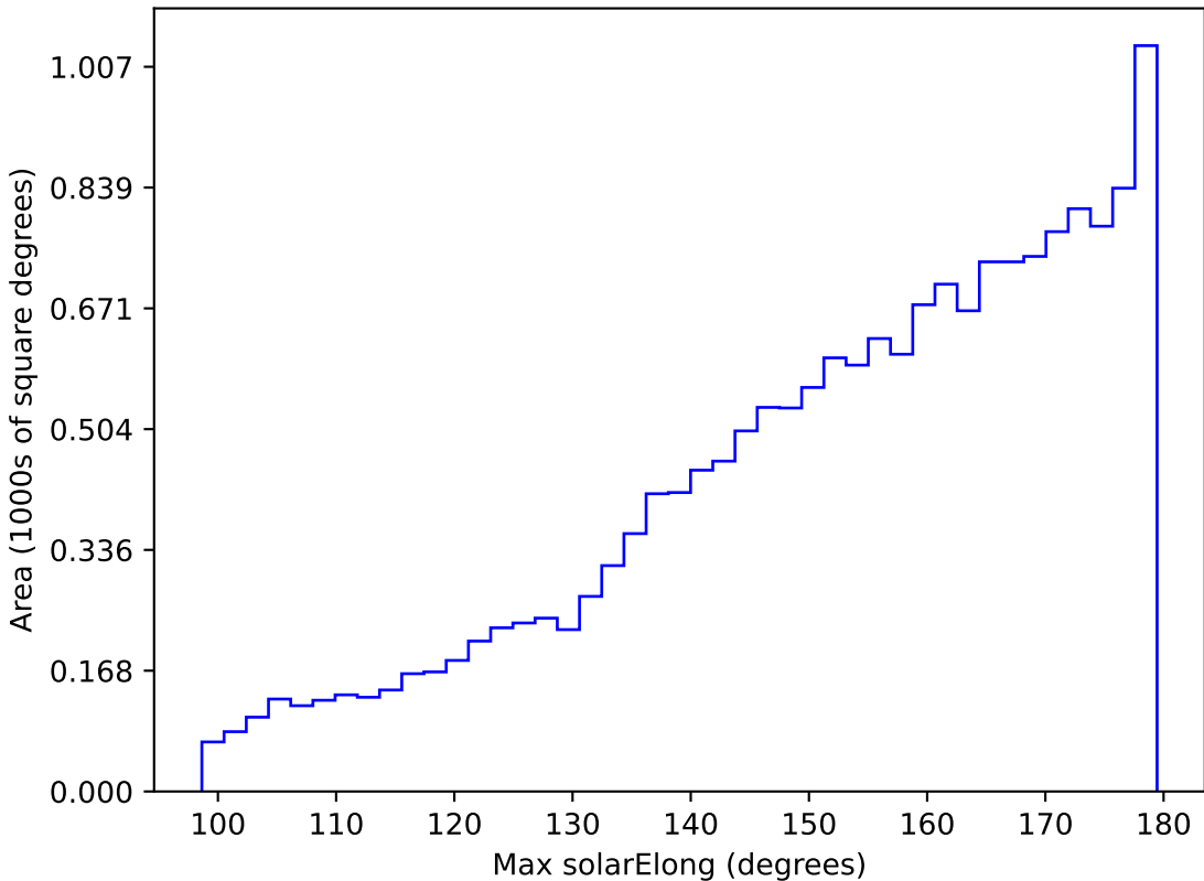
early_u_fpextra3.0_v3.4_10yrs WFD i band: Max solarElong
