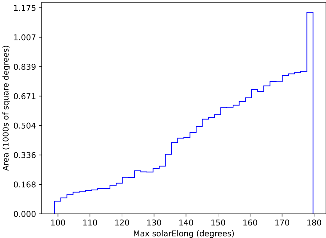
early_u_fpextra3.0_v3.4_10yrs WFD all bands: Max solarElong
