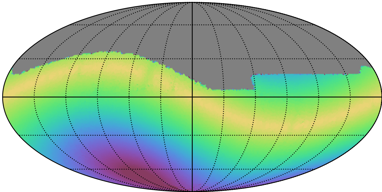
early_u_fpextra3.0_v3.4_10yrs All sky z band: Max solarElong
