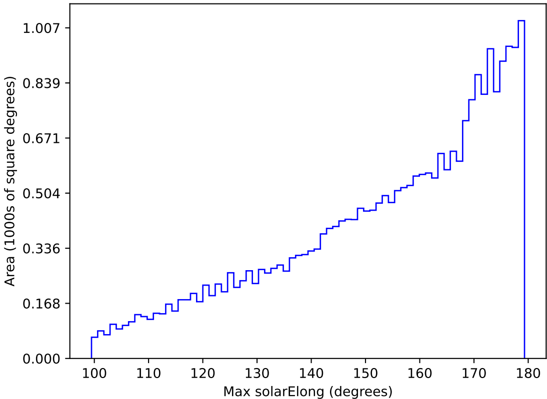
early_u_fpextra3.0_v3.4_10yrs All sky z band: Max solarElong
